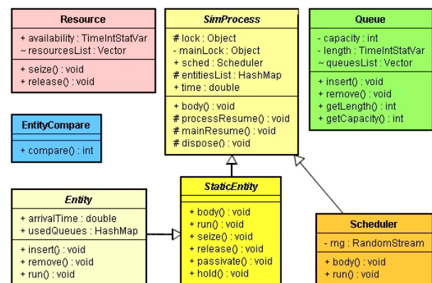
Figure 1. The Kernel class diagram.
