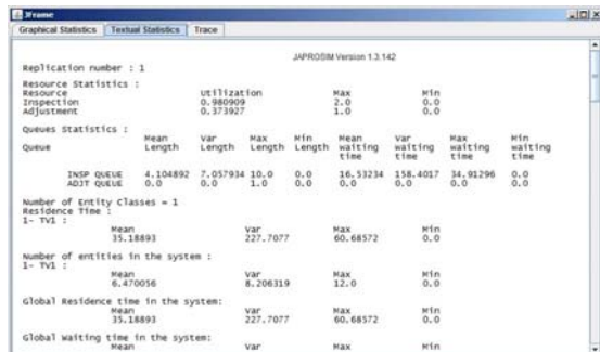
Figure 8. Statistical results.
