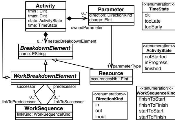
Figure 3: xSPEM metamodel (simplified)
