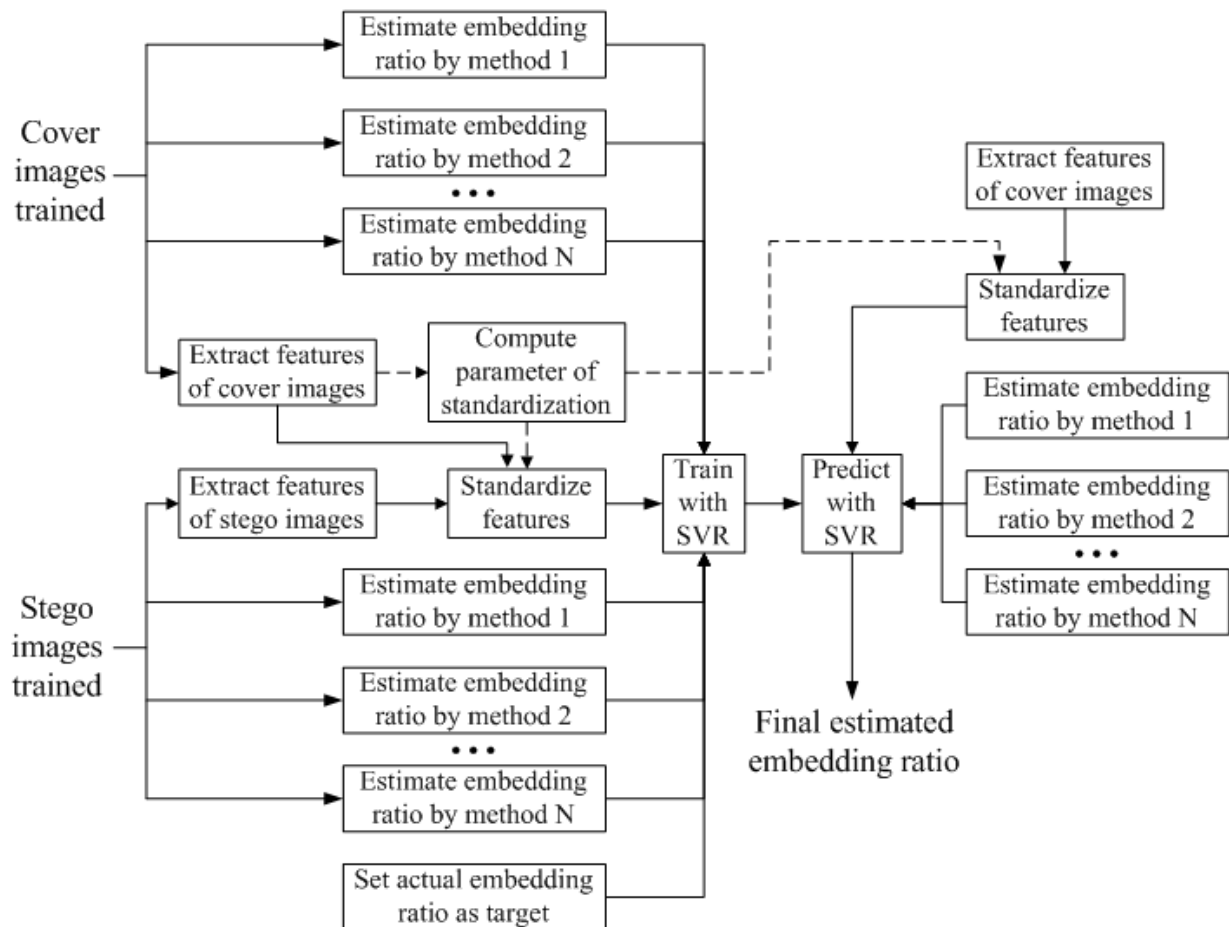
Figure 1. Diagram of the fusion method of different quantitative steganalysis methods based on SVR.
