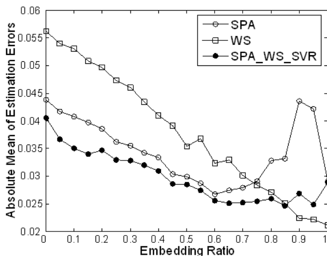
Figure 4. Absolute mean of the estimation errors of the fusion method, SPA method and WS method.
