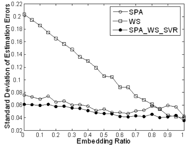
Figure 3. Standard deviation of the estimation errors of the fusion method, SPA method and WS method.
