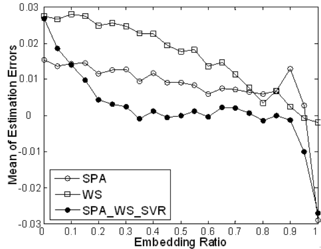
Figure 2. Mean of the estimation errors of the fusion method denoted by SPA.WS.SVR, SPA method and WS method.
