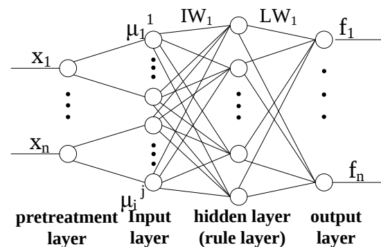
Fig. 2. Structure of fuzzy neural network
