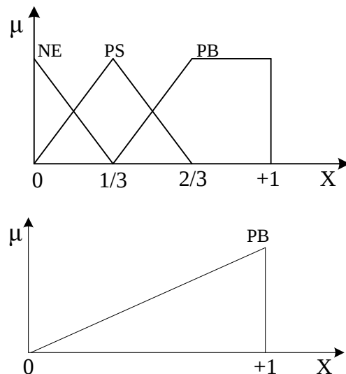
Fig 3 . Normalized graphics of fuzzy input division
