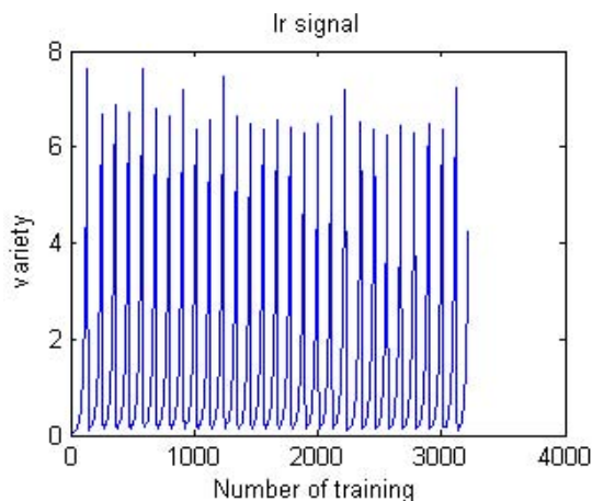
Fig 6. Learning velocity curve
