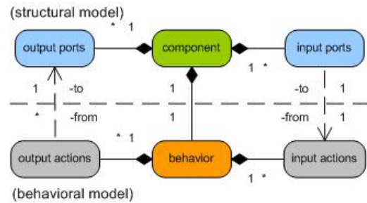
Fig. 9. Conceptual model of integrating behavioral and structural DSMLs.
