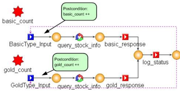
Fig. 7. Example CBML behavioral model with variables.
