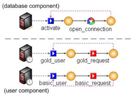
Fig. 8. CBML's domain-specific extensions to I/O automata
