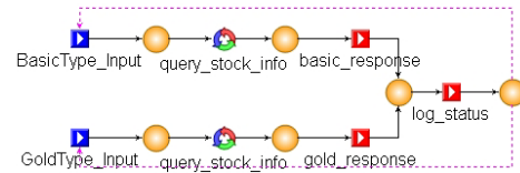
Fig. 6. Example CBML behavioral model with output actions.
