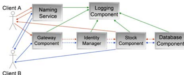
Fig. 1. High-level structural composition of the Distributed Stock Application.
