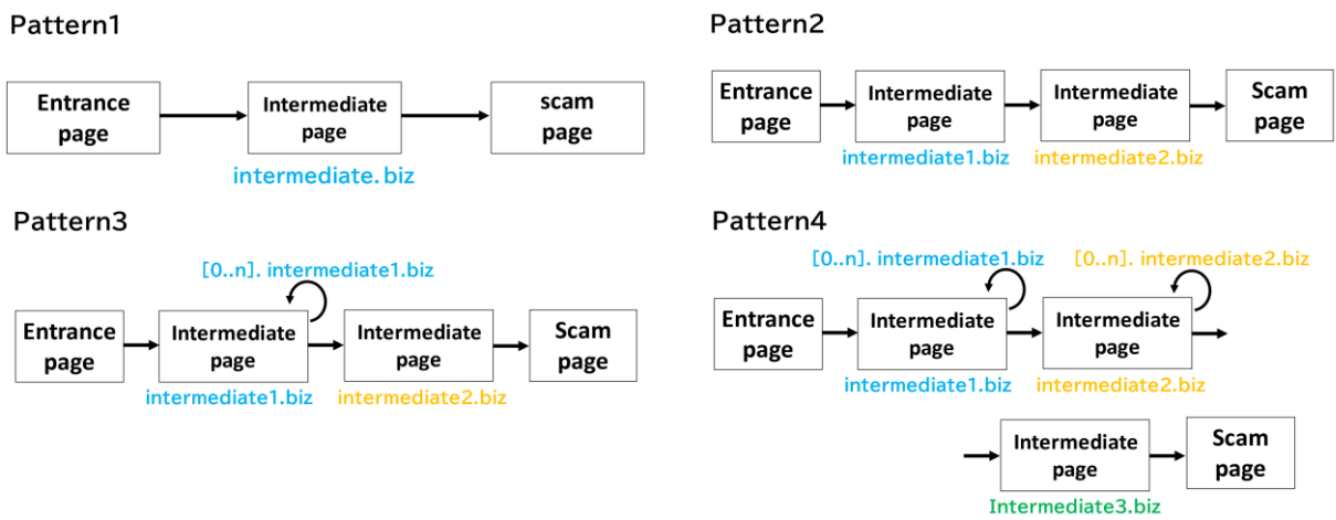
Fig. 2. Example of each pattern operation.
